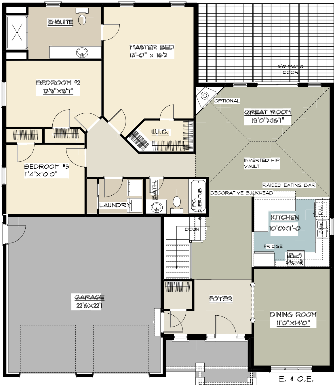
GROUND FLOOR PLAN 1763 SQ FT
